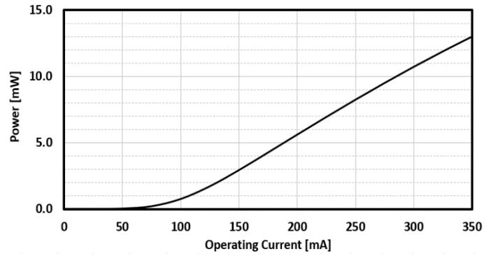
FIG. 2: BTF PACKAGE OUTPUT POWER VS CURRENT
