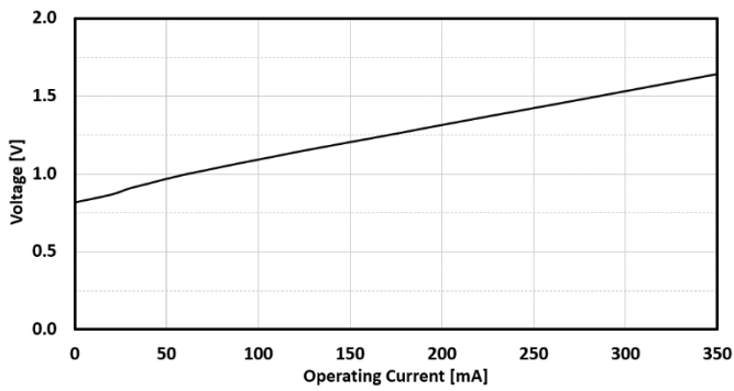
FIG. 3: BTF PACKAGE FORWARD VOLTAGE VS CURRENT
