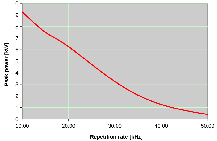
Wedge XF 266nm: Peak Power
