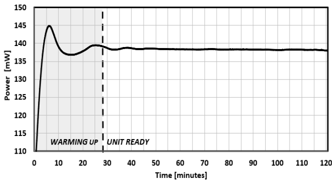
FIG. 15: WARM-UP TIME
