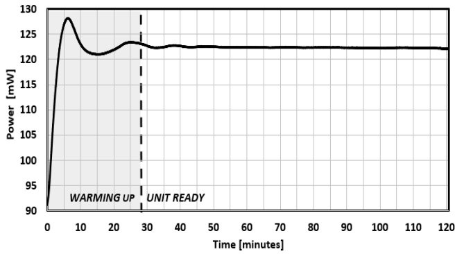
FIG. 13: WARM-UP TIME
