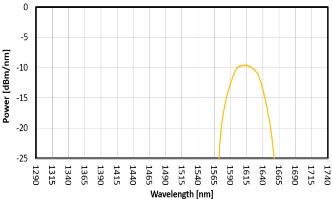
FIG. 5: SLED 4 SPECTRUM
