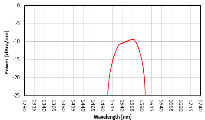
FIG. 6: SLED 5 SPECTRUM
