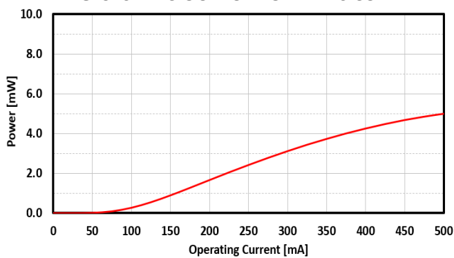
FIG. 11: SLED 5 OUTPUT POWER VS CURRENT
