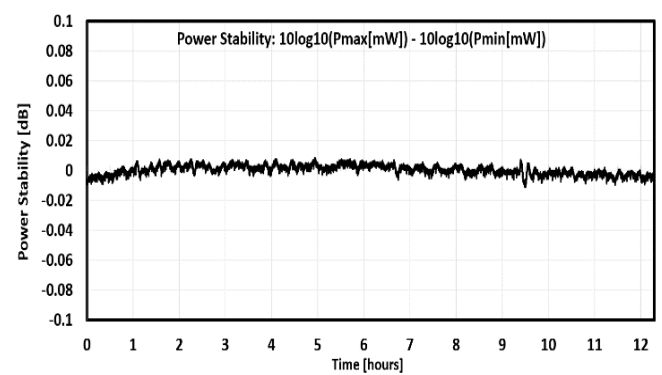
FIG. 10: ISB2 TYPICAL POWER STABILITY
