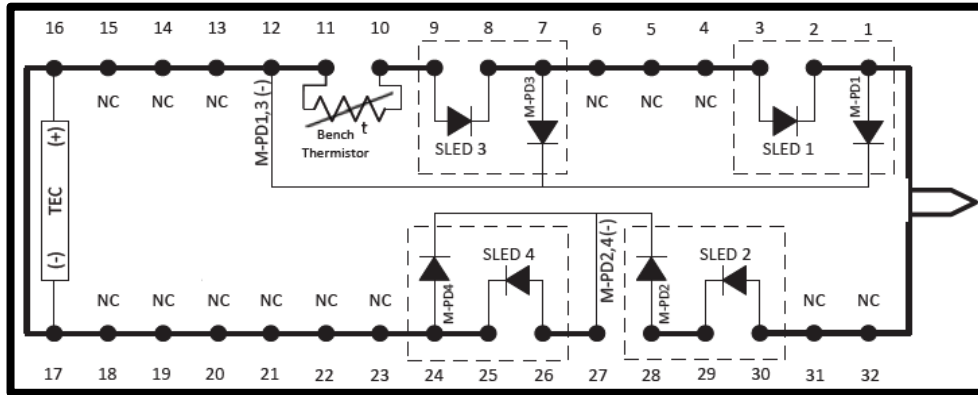
External Pin Assignment – BeST-SLED: 4 SLEDs
