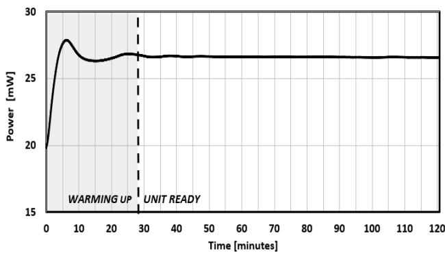
FIG. 11: WARM-UP TIME
