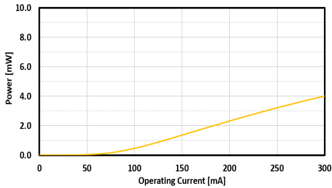
FIG. 7: SLED 2 OUTPUT POWER VS CURRENT
