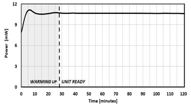
FIG. 10: WARM-UP TIME
