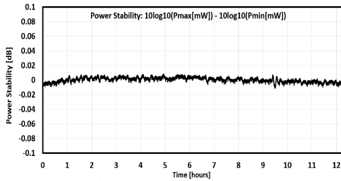
FIG. 9: OSE2 TYPICAL POWER STABILITY
