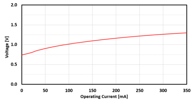
FIG. 16: SLED 3 FORWARD VOLTAGE VS CURRENT
