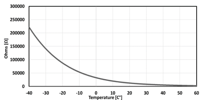
FIG. 20: THERMISTOR R THTEC RESISTANCE VS TEMPERATURE
