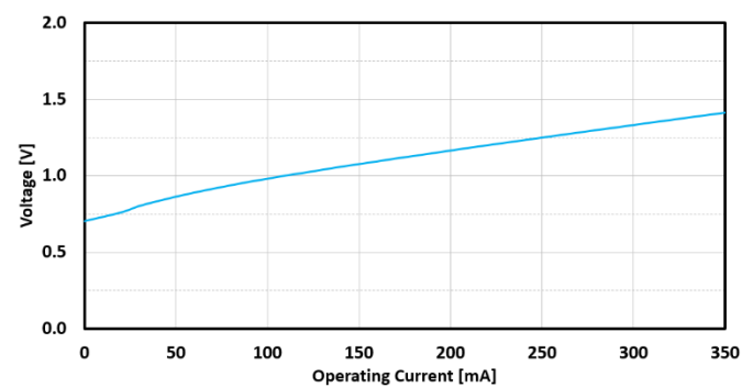
FIG. 18: SLED 5 FORWARD VOLTAGE VS CURRENT
