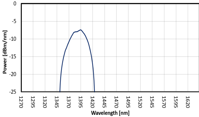
FIG. 5: SLED 4 SPECTRUM
