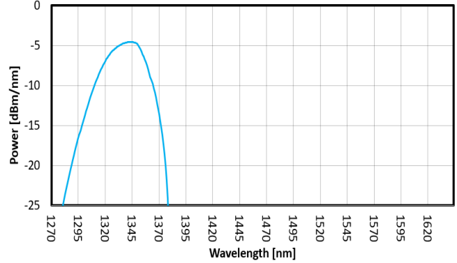
FIG. 6: SLED 5 SPECTRUM
