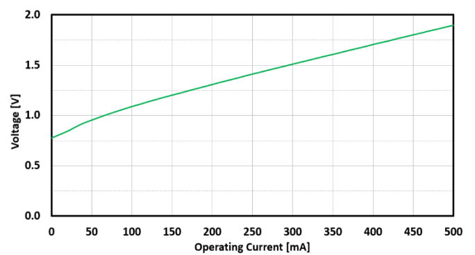
FIG. 14: SLED 3 FORWARD VOLTAGE VS CURRENT
