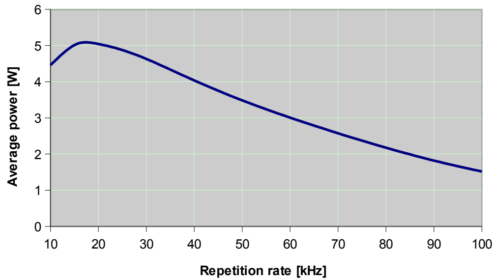
Sol 5W 532nm: Average Power
