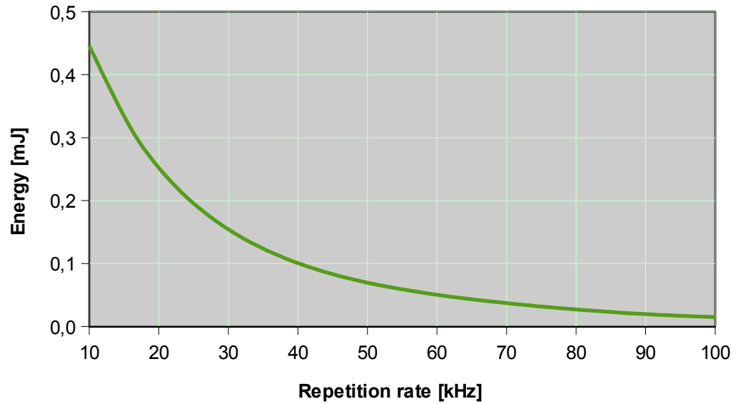
Sol 5W 532nm: Pulse Energy
