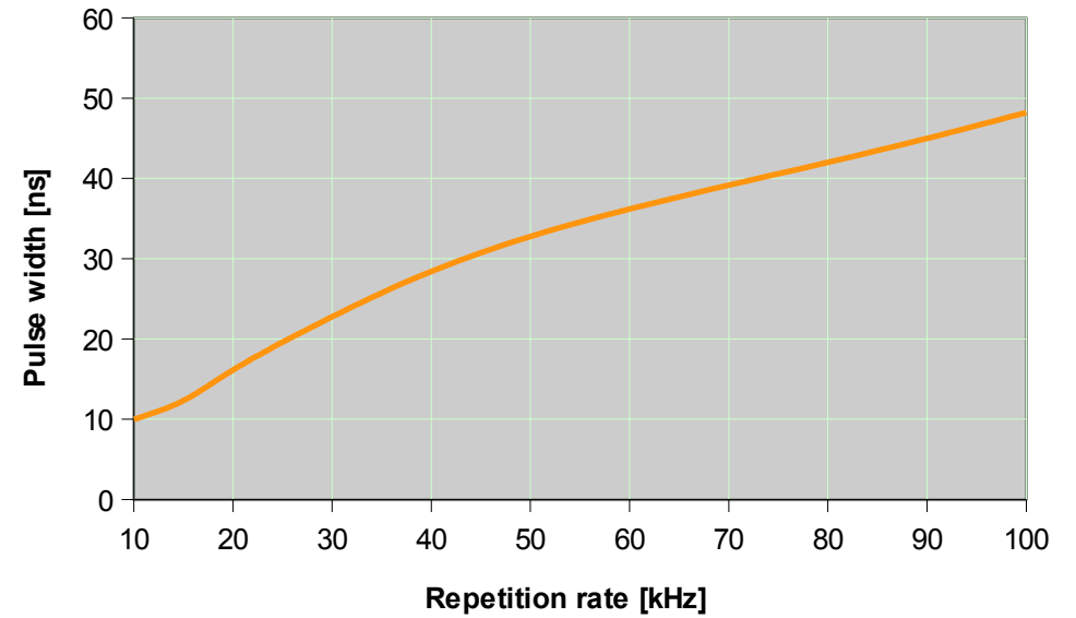
Sol 5W 532nm: Pulse Width
