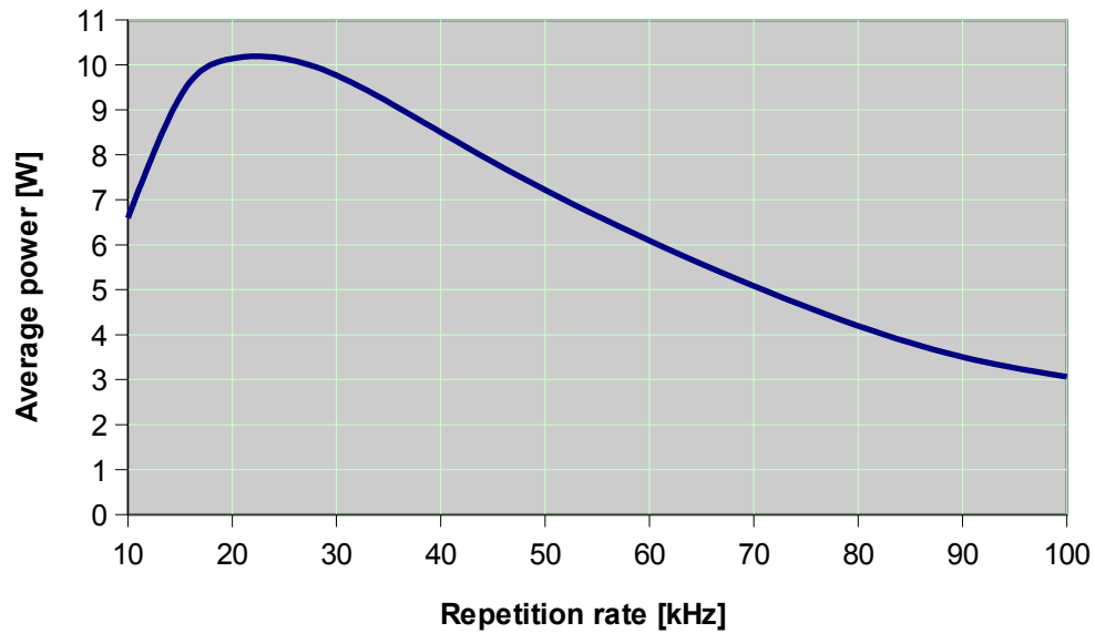
Sol 10W 532nm: Average Power
