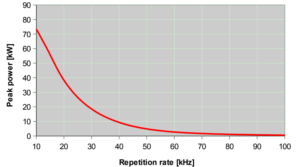
Sol 10W 532nm: Peak Power
