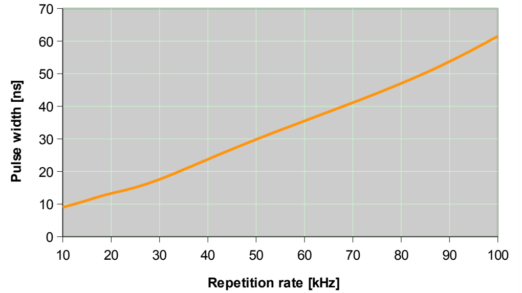
Sol 10W 532nm: Pulse Width
