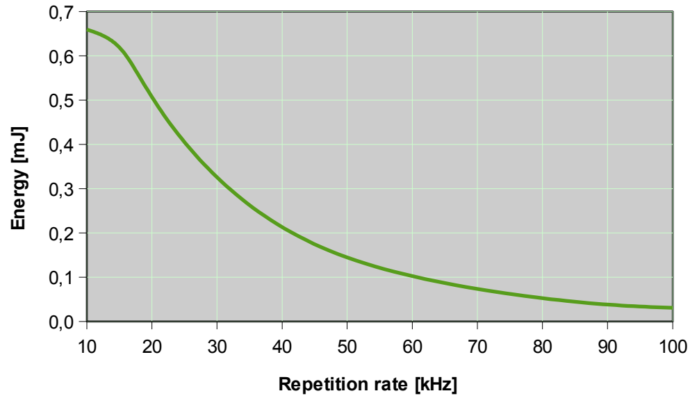
Sol 10W 532nm: Pulse Energy
