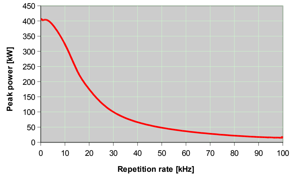
Onda 1064nm: Peak Power
