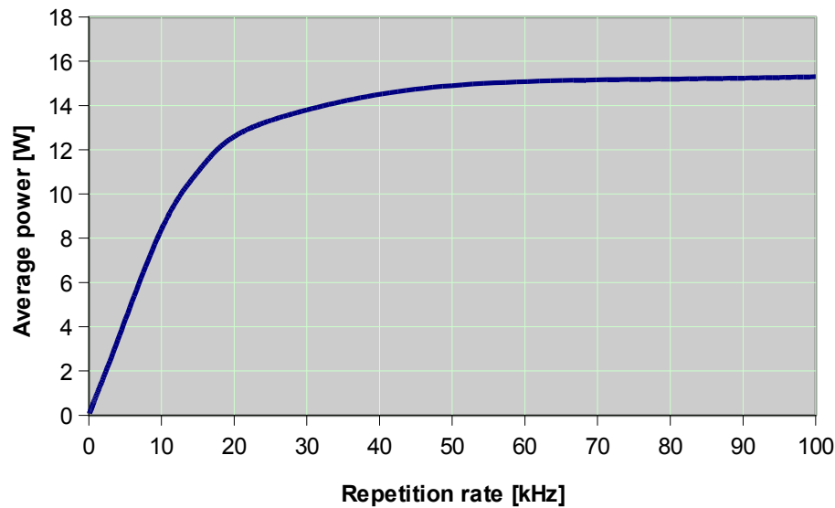
Onda 1064nm: Average Power
