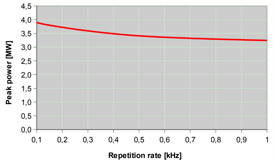
Wedge XB 1064nm: Peak Power
